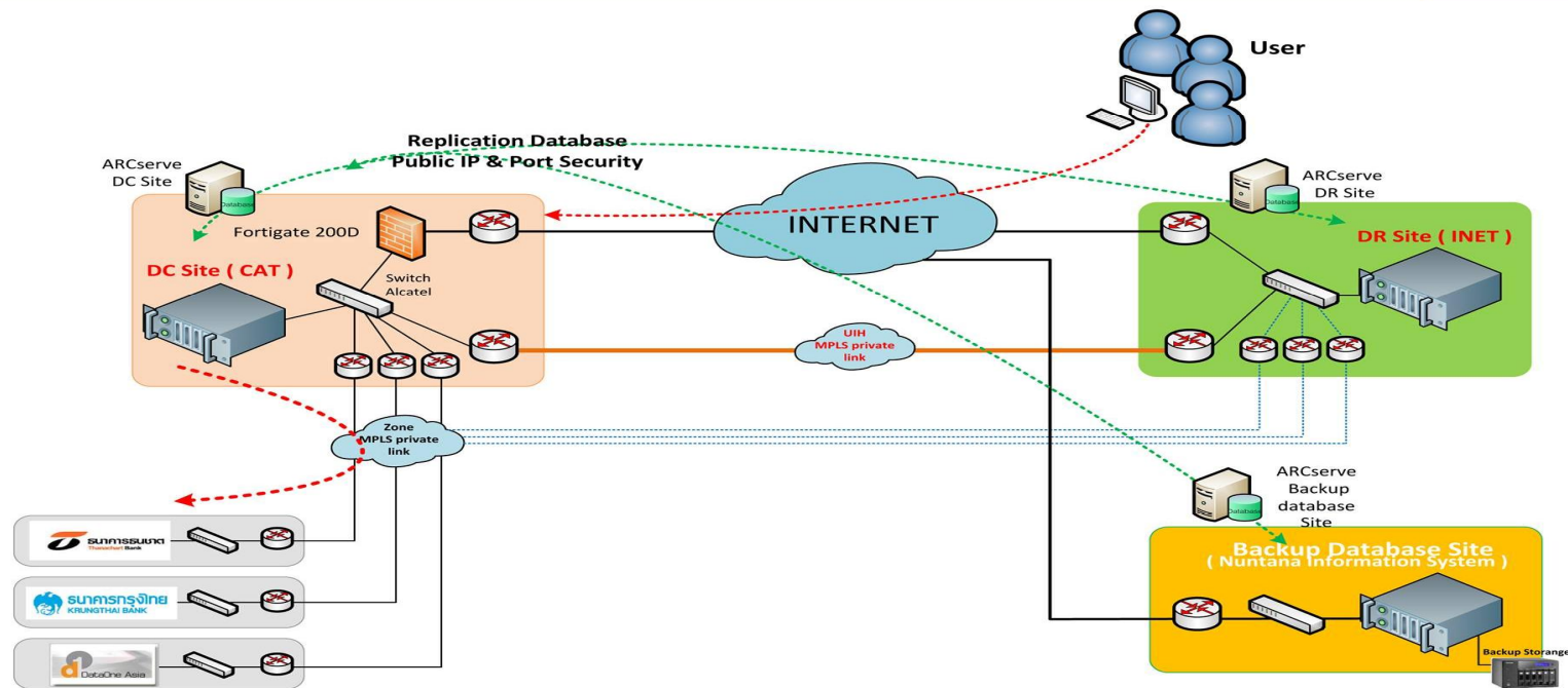
Network Diagram Nuntana Information System : DC Site & DR Site
