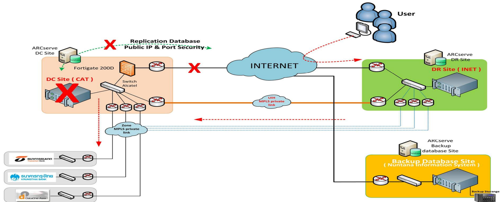
Network Diagram Nuntana Information System : Sever DC Site & link Down
